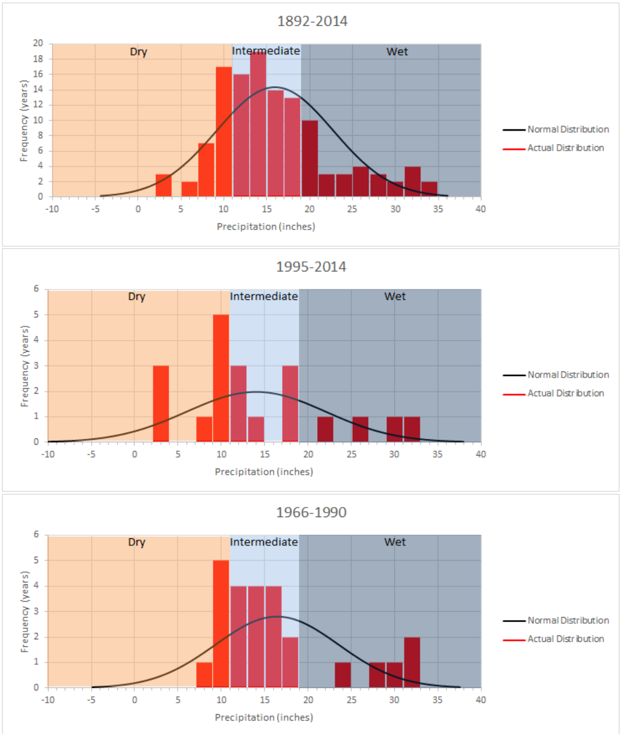
Figure 2. Frequency distribution curves and water year type designations for 1892-2014, 1995-2014 and 1966-1990 periods based on San Bernardino Hospital Gage precipitation data.
