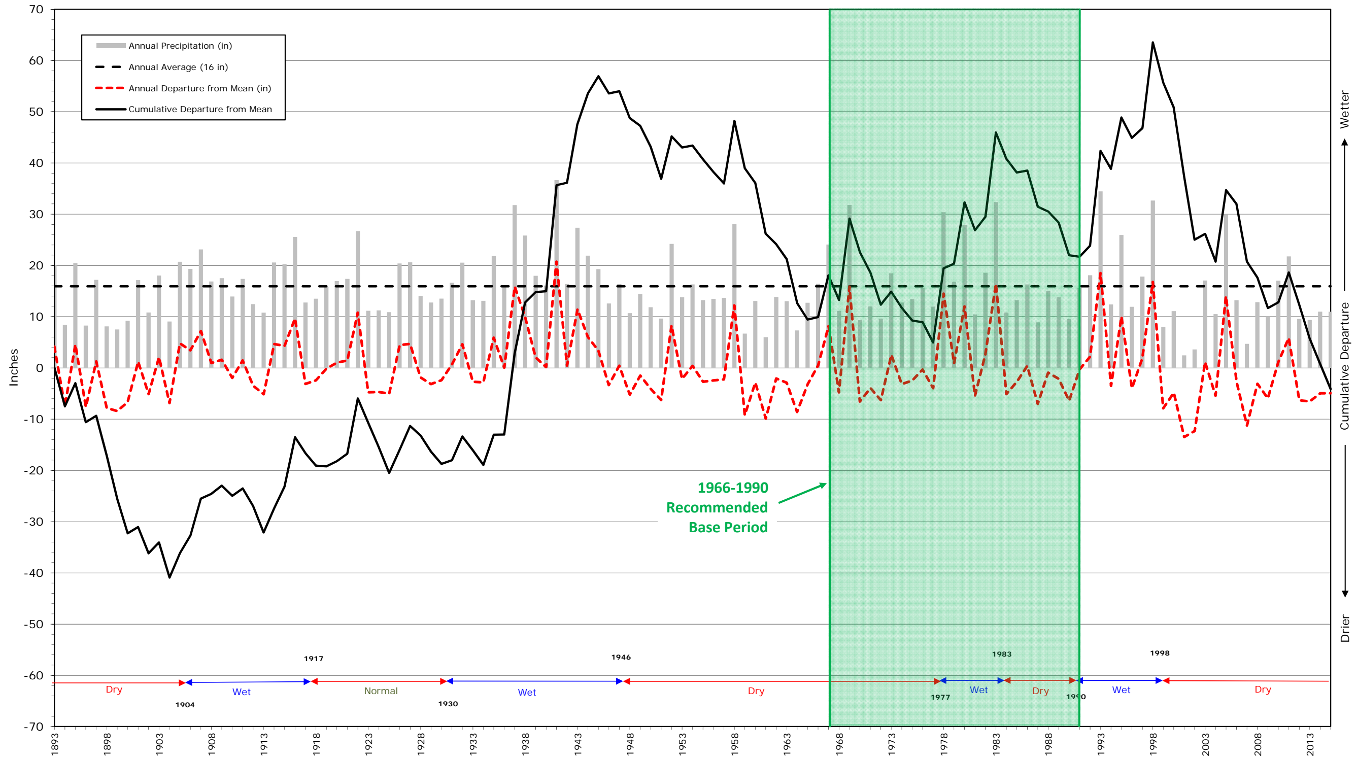
Figure 1. San Bernardino Hospital Gage cumulative precipitation departure analysis from 1892-2014. Source: Farid Boushaki, Riverside Public Utilities.
